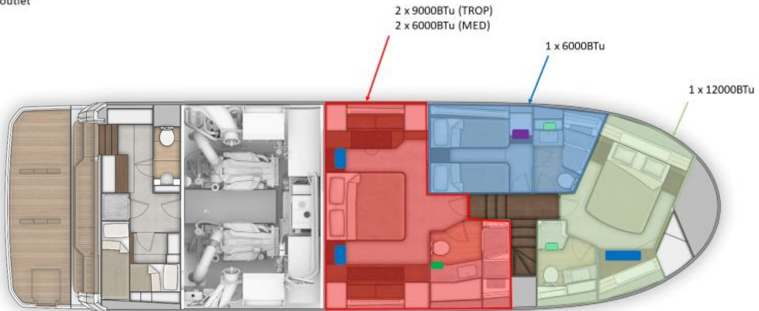
LOWER ACCOMMODATION PLAN - 3 CABIN LAYOUT
